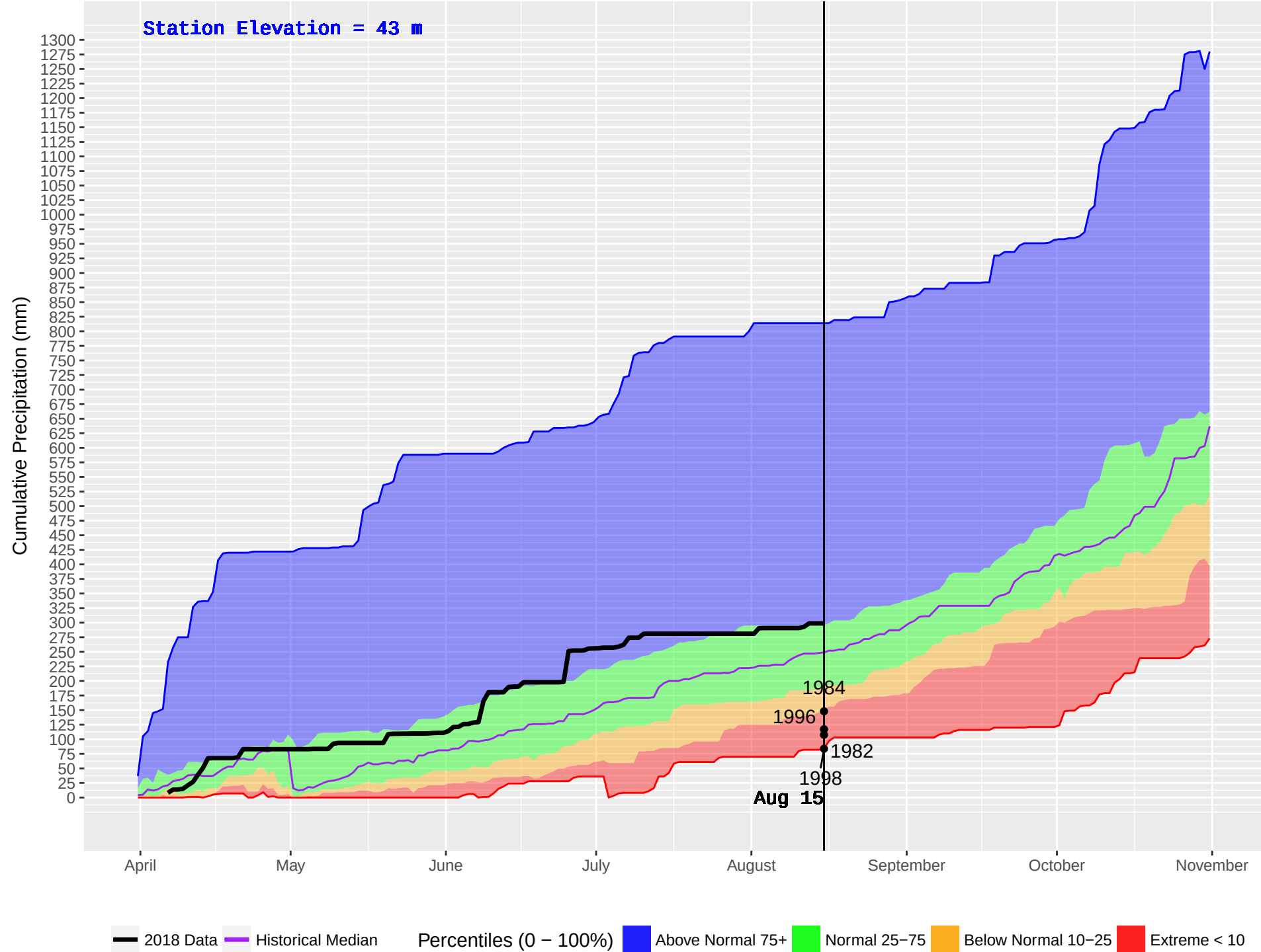
TOBA CAMP (75) : Historical (1970–2016) and Current (2018) Daily Cumulative Precipitation
