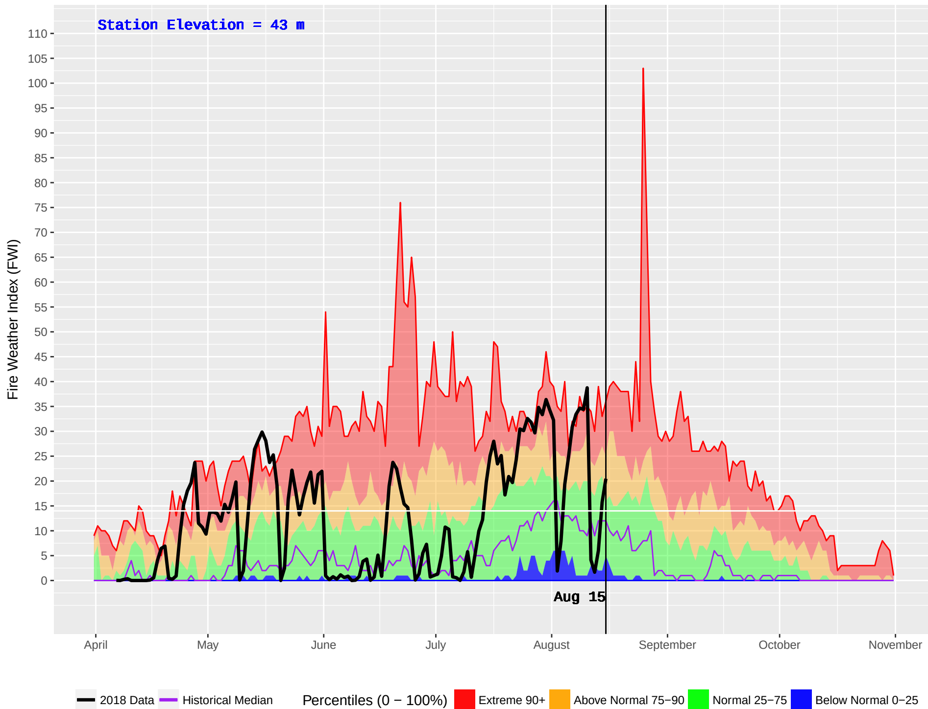
TOBA CAMP (75) : Historical (1970–2016) and Current (2018) Daily Fire Weather Index (FWI)
