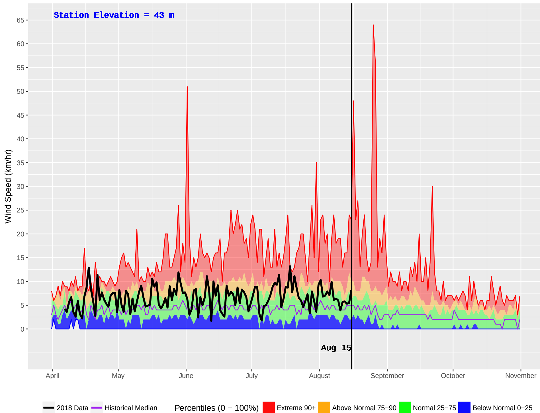
TOBA CAMP (75) : Historical (1970–2016) and Current (2018) Daily Wind Speed
