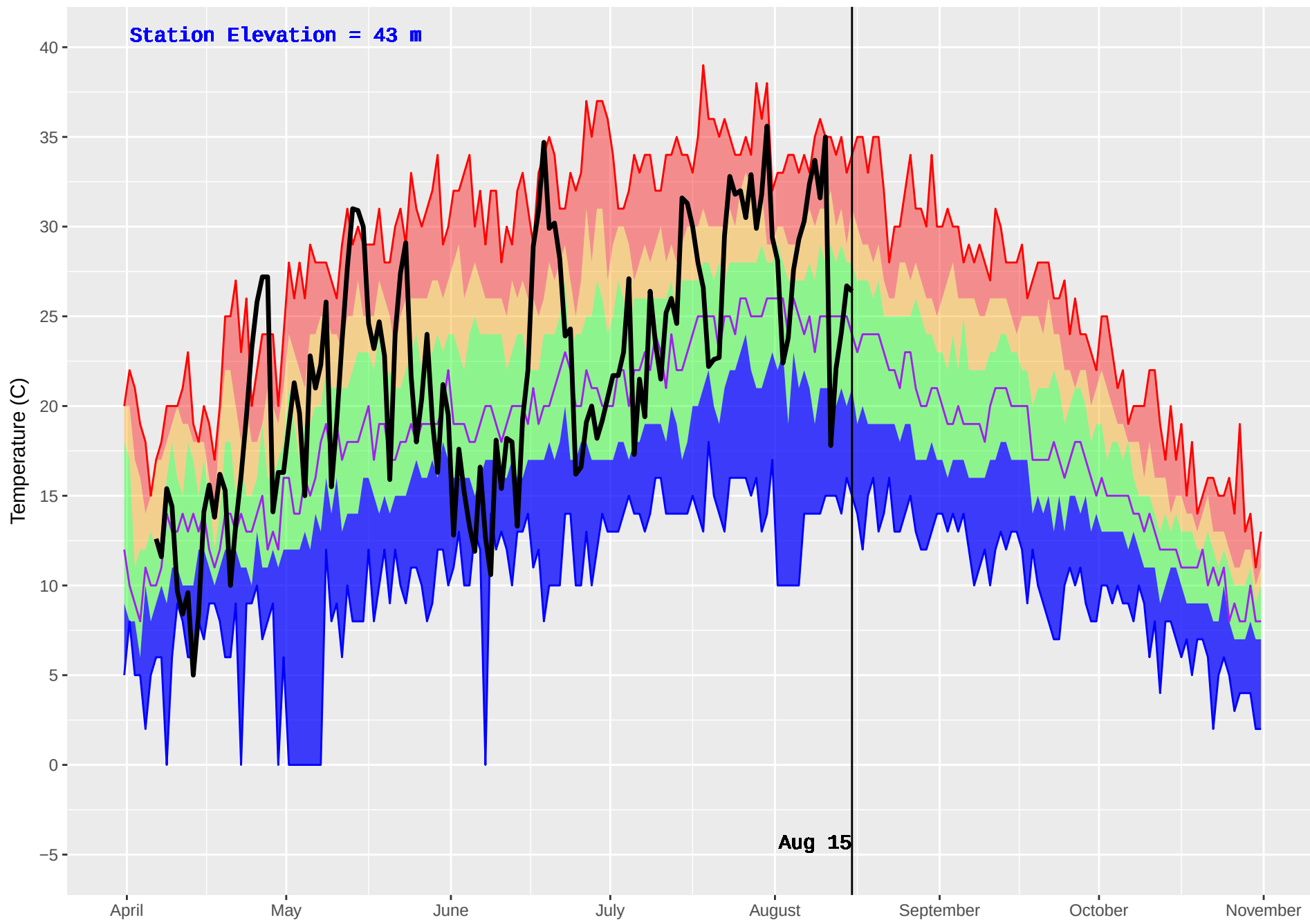
TOBA CAMP (75) : Historical (1970–2016) and Current (2018) Daily Temperature
